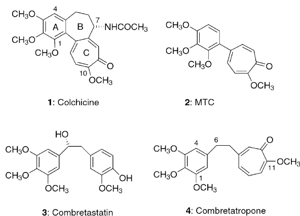
Figure 1. Structures of colchicine and analogues.
