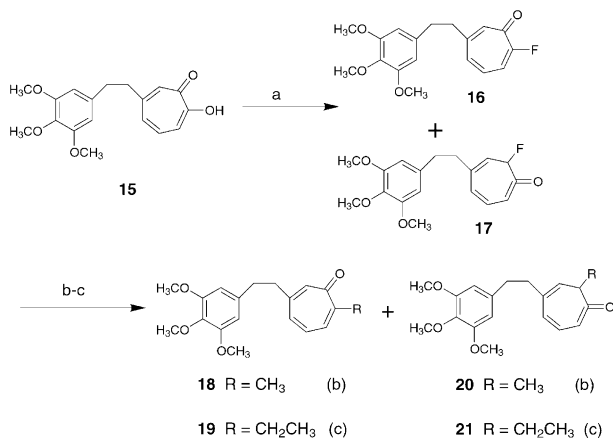
Scheme 3. (a) DAST, CH 2 Cl 2 , 83%; (b) CH 3 MgBr, THF, 0 °C; (c) CH 3 CH 2 MgBr, THF, 0 °C.
