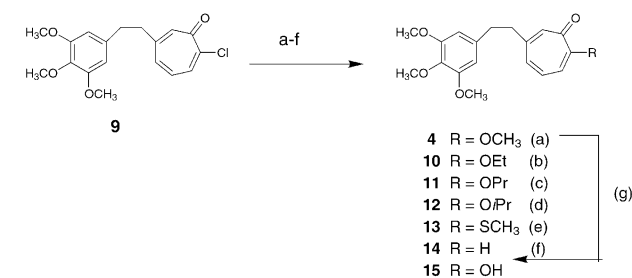
Scheme 2. (a) Mg, I 2 , CH 3 OH, 66%; (b) EtOH, EtMgBr, THF, 73%; (c) PrOH, PrMgBr, THF, 76%; (d) Na, i PrOH, 38%; (e) NaSCH 3 , H 2 O, CH 3 OH, 78%; (f) NaBH 4 , DMSO, 67%; (g) 2 N HCl, CH 3 OH, reflux, 86%.
