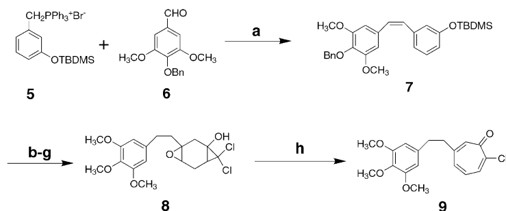
Scheme 1. (a) n BuLi, THF, 58%; (b) H 2 , Pd/C, EtOH, 96%; (c) Li/NH 3 , t -BuOH, THF, reflux, 90%; (d) CH 2 N 2 , CH 2 Cl 2 , 97%; (e) NaO 2 C 2 Cl 3 , DME, reflux; (f) 20% HF, CH 3 CN, 53%; (g) m CPBA, CH 2 Cl 2 , 67%; (h) pTSA, C 6 H 6 , reflux, 57%.
